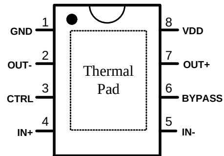
Top View HT6881D2SDE (DFN8L)
